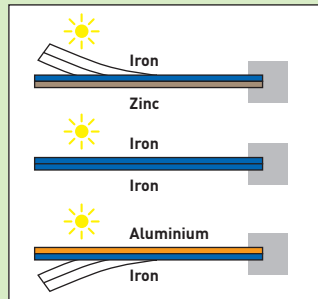
Illustration of the bimetal effect when exposed to temperature fluctuations
