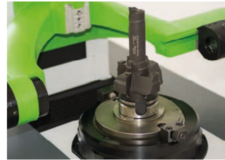
Modular precision spindle the most stable and precise tool holder spindle.
