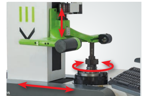
Autofocus / CNC · The axes (C, X, Z) can optionally be motor-actuated for automatic measuring processes · Equally feasible – Autofocus only
